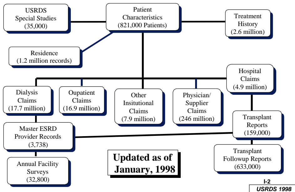
Overall structure of the USRDS database with counts of patient and facility records as of January, 1998.
